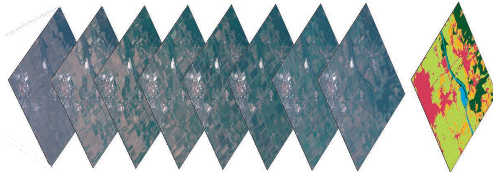
CLOUD MASK
